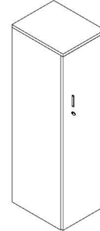
Gabinete Alto Closet 1P F: 37,5/40/45 P: 55 H: 165
